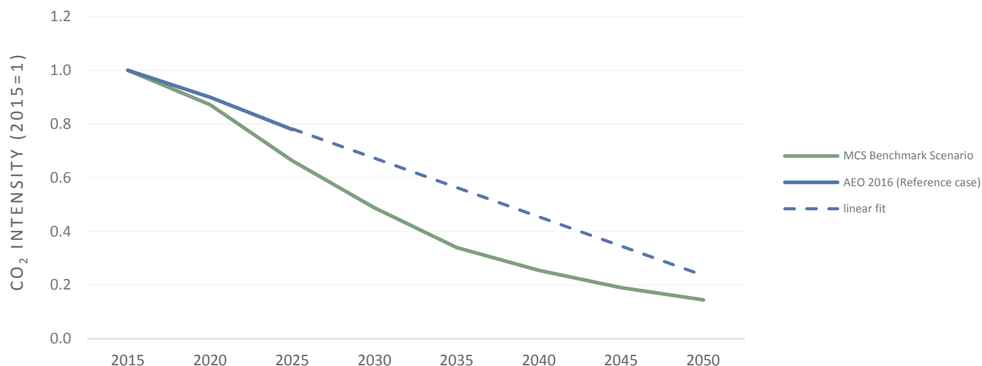
FIGURE 4.11: FLEET-WIDE EMISSIONS INTENSITY FOR LIGHT-DUTY VEHICLES UNDER THE MCS BENCHMARK SCENARIO RELATIVE TO A STRAIGHT-LINE EXTENSION OF NEAR-TERM PROJECTIONS TO 2025
