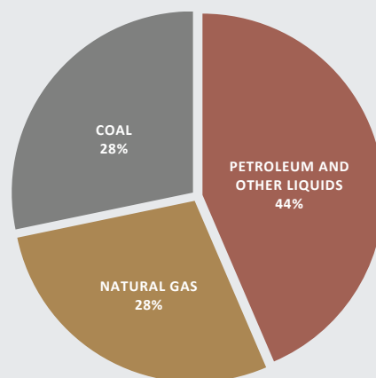
FIGURE 4.1: U.S. CO 2 EMISSIONS FROM ENERGY CONSUMPTION BY FUEL, 2015 (EIA 2016D)
