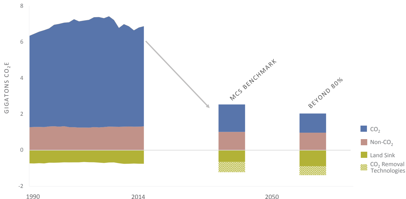
FIGURE 3.4: COMPONENTS OF ILLUSTRATIVE “BEYOND 80” SCENARIO
