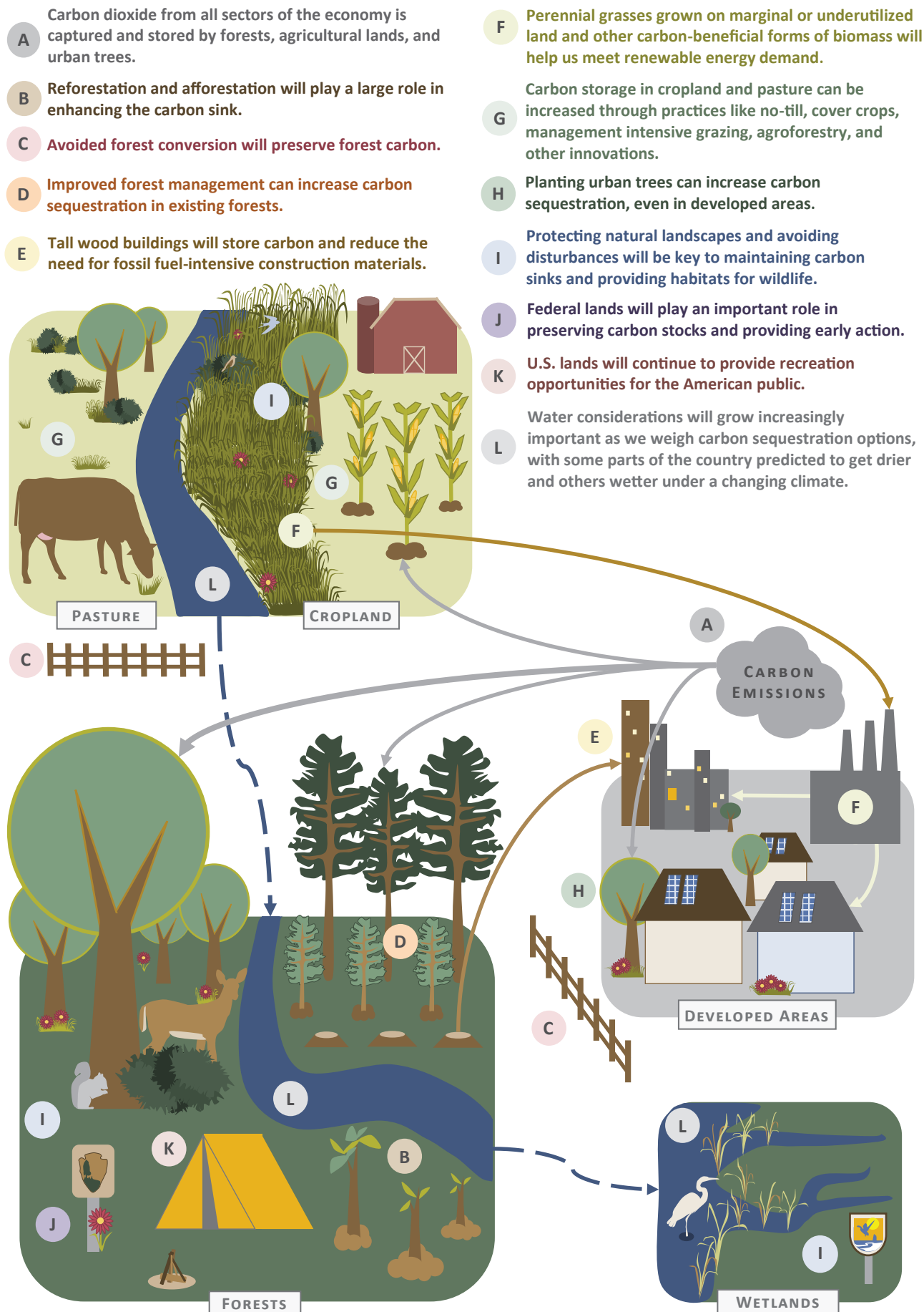
FIGURE 5.2: ROLE OF U.S. LANDS IN THE MID-CENTURY STRATEGY
