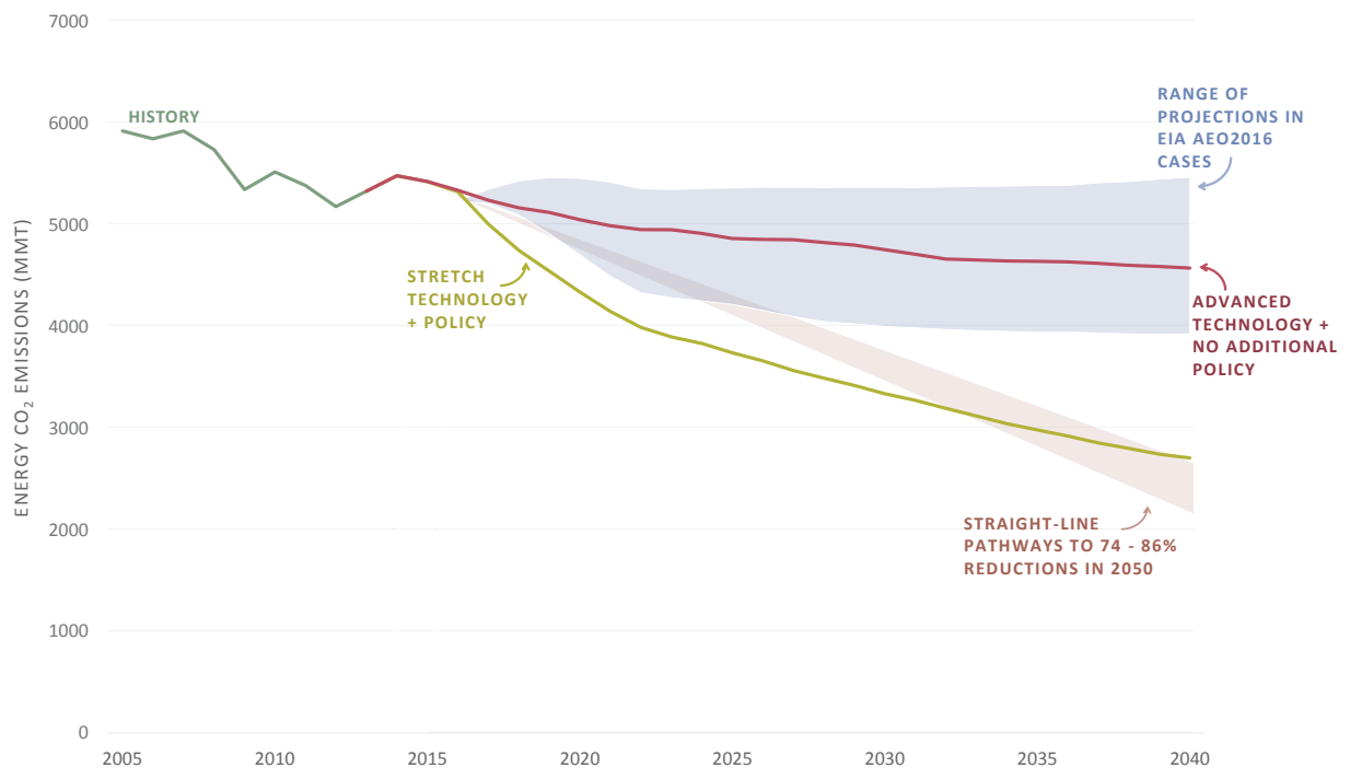
FIGURE E3: ENERGY CO 2 EMISSIONS UNDER CURRENT AND EXPANDED AMBITION POLICIES
