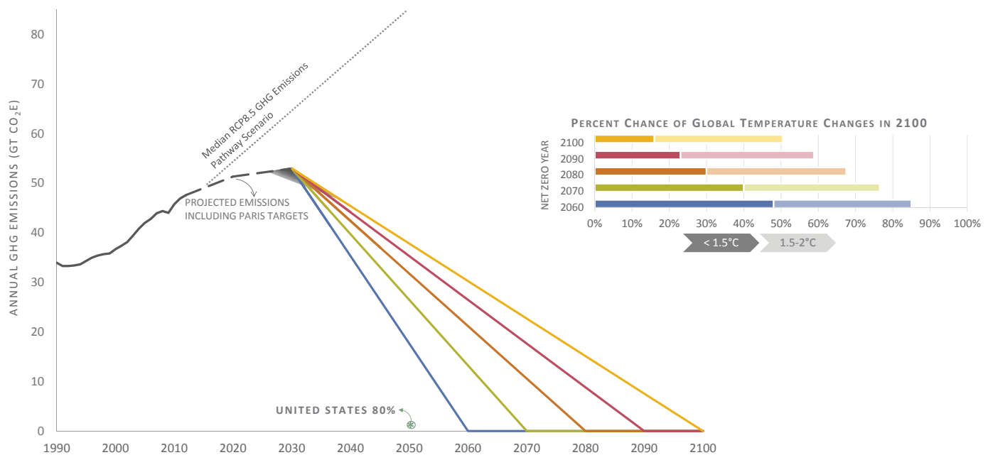
FIGURE 7.2: GLOBAL GHG EMISSIONS AND TEMPERATURE CHANGES UNDER DIFFERENT NET-ZERO EMISSIONS SCENARIOS
