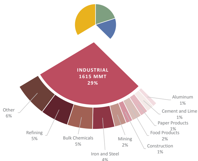
FIGURE 4.16: CO 2 EMISSIONS BY END USE: INDUSTRIAL
