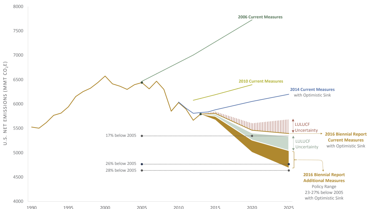
FIGURE 2.3: U.S. EMISSIONS PROJECTIONS WITH CURRENT MEASURES AND ADDITIONAL MEASURES CONSISTENT WITH OBAMA ADMINISTRATION'S CLIMATE ACTION PLAN (U.S. DEPARTMENT OF STATE 2016)
