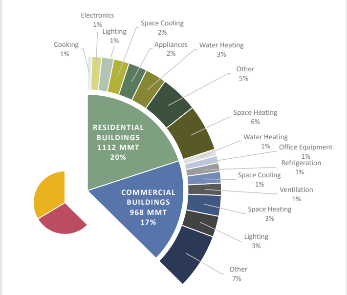
FIGURE 4.13: CO 2 EMISSIONS BY END USE: BUILDINGS
