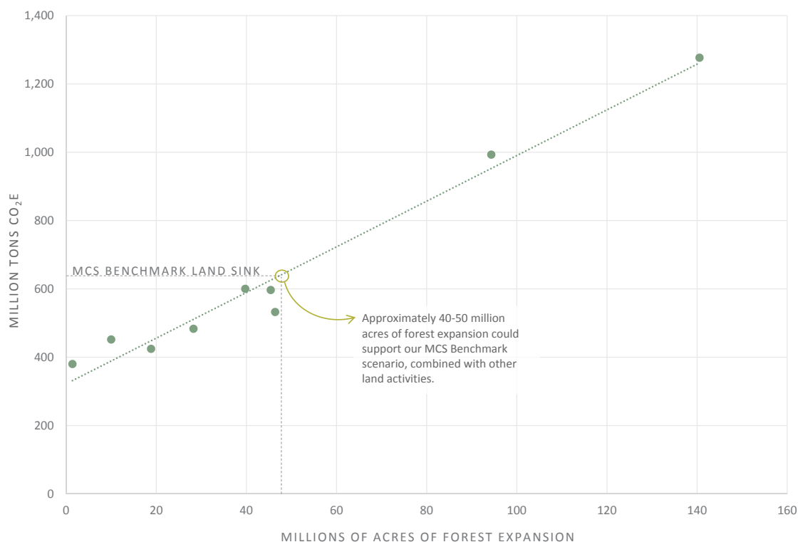
FIGURE 5.3: CUMULATIVE AFFORESTATION AND AVERAGE ANNUAL CO 2 STOCK CHANGE
