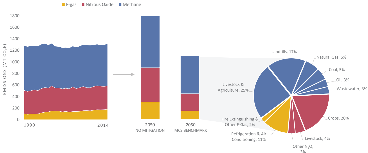
FIGURE 6.2: NON-CO 2 EMISSIONS REDUCTIONS IN 2050 WITH MCS BENCHMARK SCENARIO
