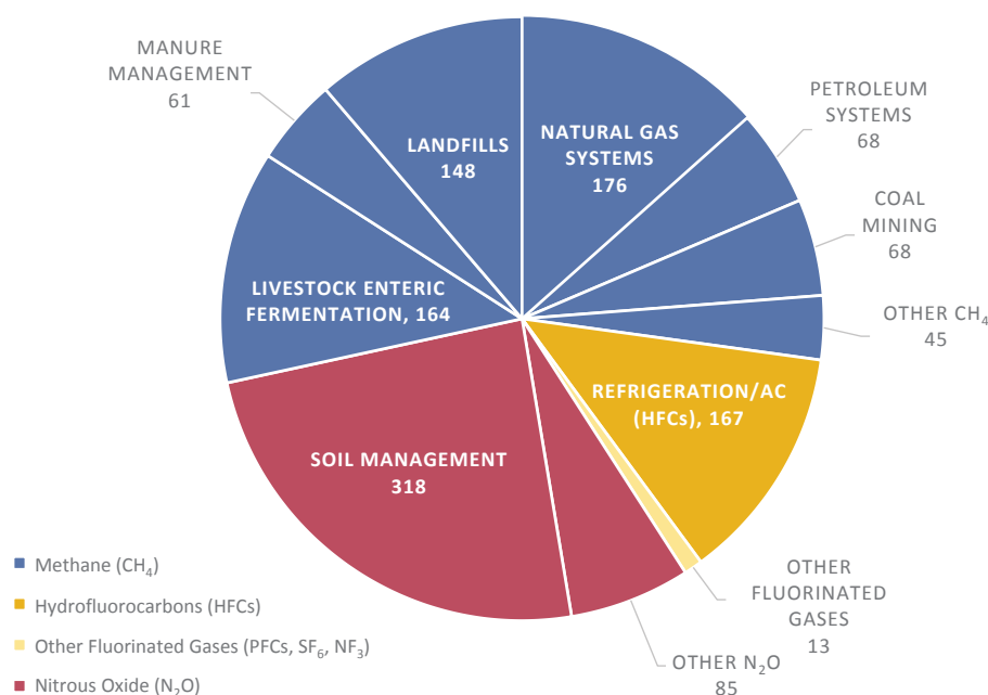
FIGURE 6.1: SOURCES OF U.S. NON-CO 2 GREENHOUSE EMISSIONS BY GAS, 2014 (MMT CO 2 E)
