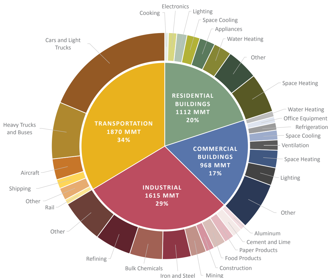
FIGURE 4.2: CO 2 EMISSIONS BY SECTOR AND END USE WITH ELECTRICITY EMISSIONS DISTRIBUTED ACROSS END-USE SECTORS, 2014
