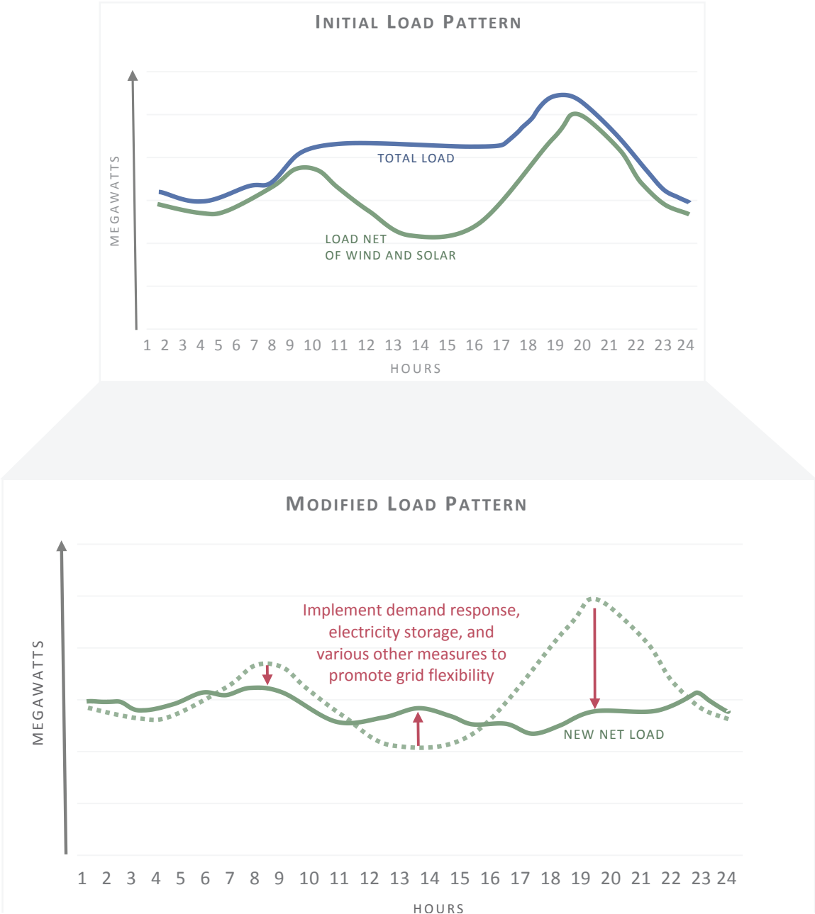
FIGURE 4.8: GRID FLEXIBILITY MEASURES TO ENABLE INCREASED VARIABLE WIND AND SOLAR PENETRATION
